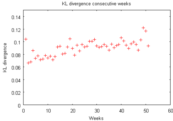
Figure 3: KL divergence between consecutive weeks.
